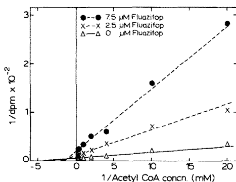
Fig. 3. Inhibition kinetics for fluazifop acid, with acetyl-CoA as the variable substrate, measured using the ^{14}C assay.
