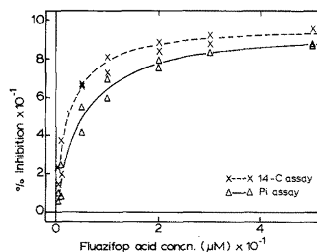
Fig. 4. IC_{50} for fluazifop acid measured using ^{14}C and phosphate assays.
